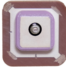
APARM2508S-SGL2L5 GPS L1 + L2 + L5 Stacked Patch Antenna
