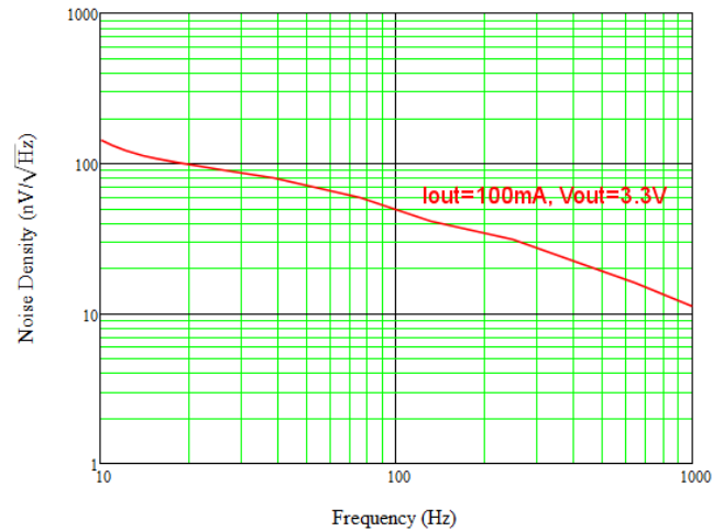
Noise Density
