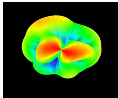
1850 MHz
