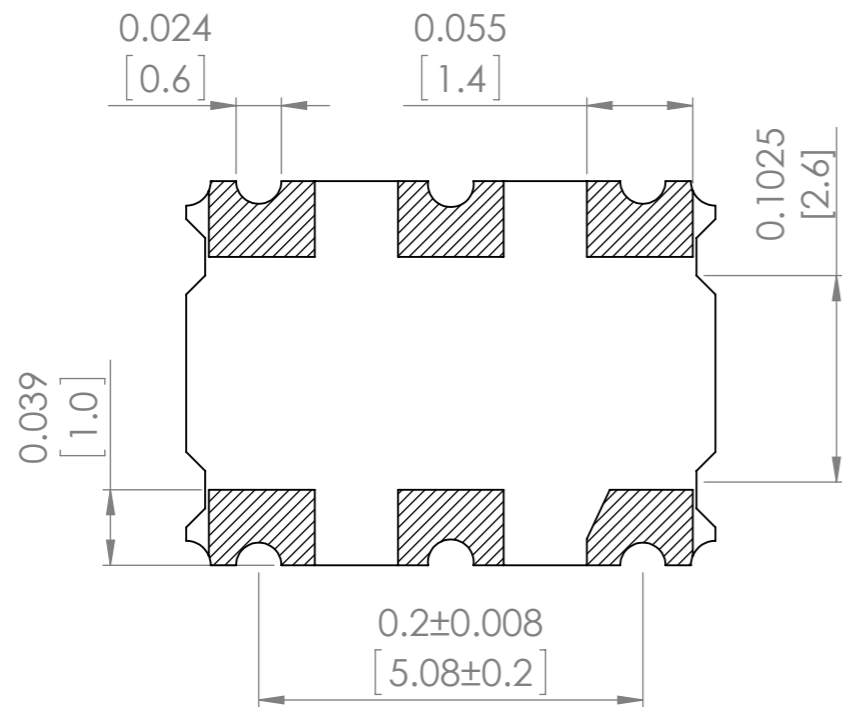
Bottom view
