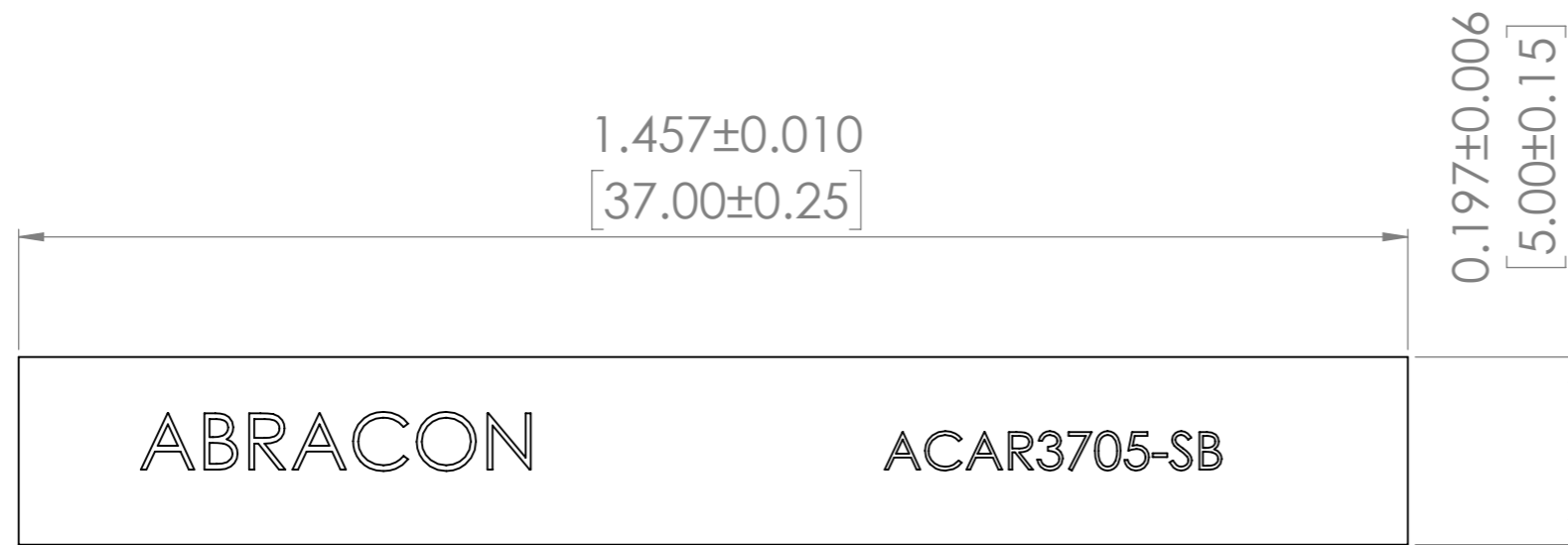
TOP VIEW
