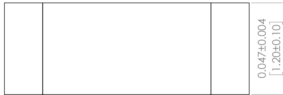
SIDE VIEW
