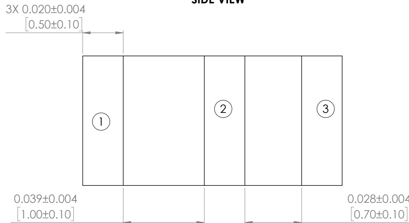
BOTTOM VIEW
